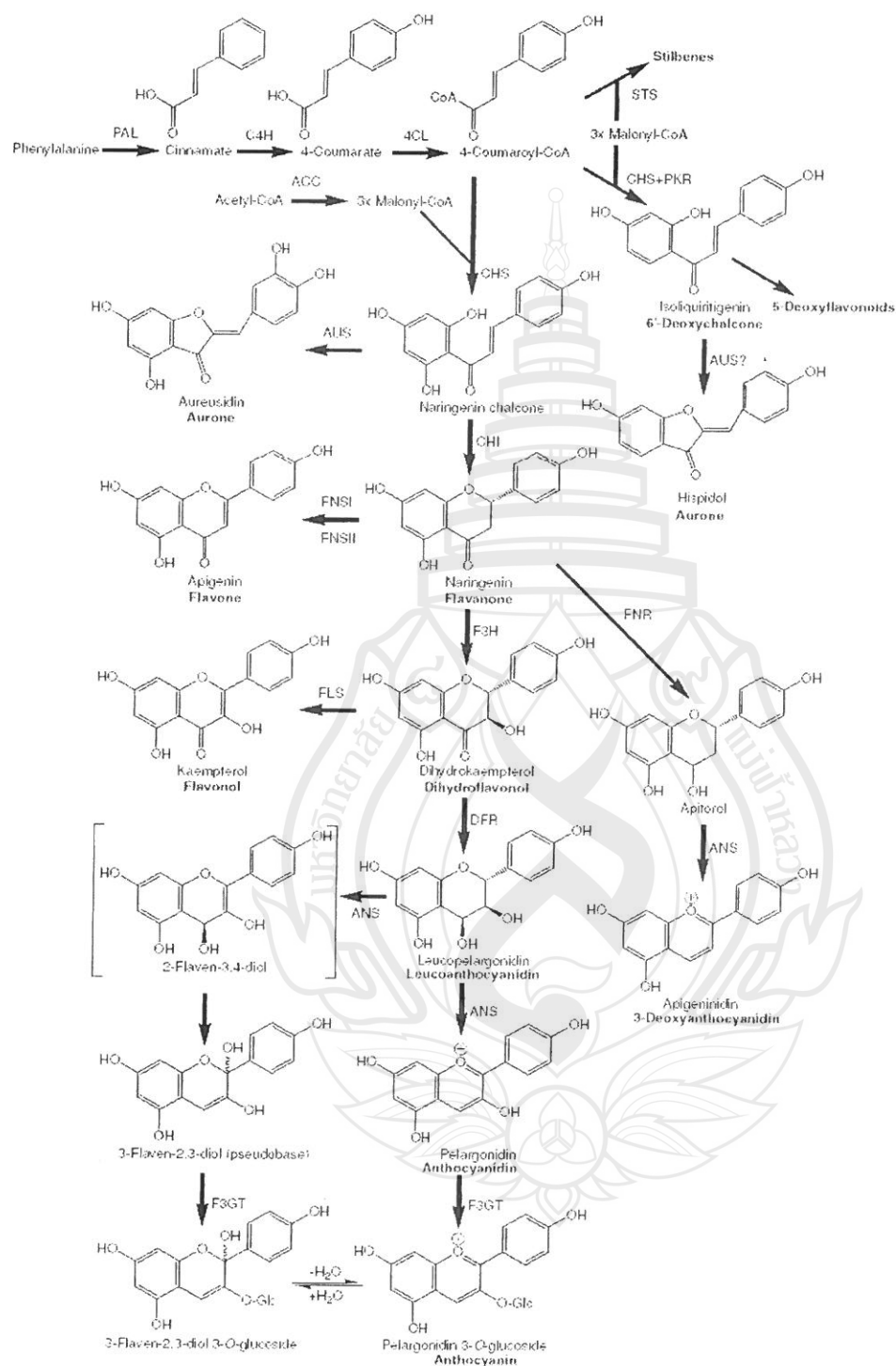
Figure 2.6: The pathway of flavonoid synthesis (Vermerris and Nicholso, 2006)
