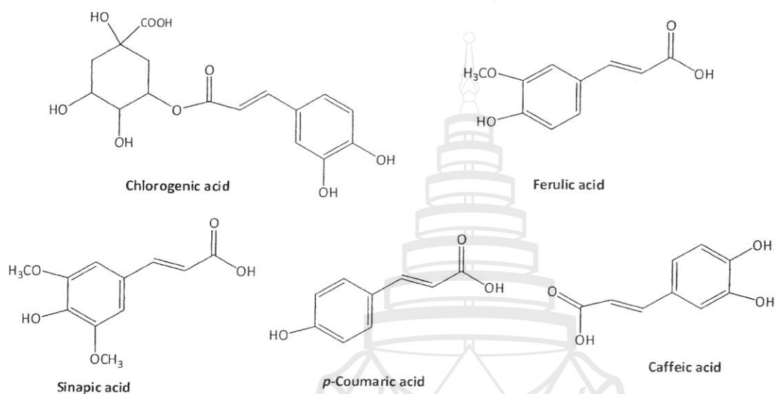
Figure 2.11: The structures of phenolic compounds in pummelos and grapefruits
