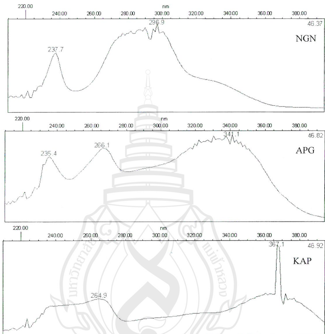
Figure 4.13: Spectrum of eight flavonoid standards by UV-visible scanning
