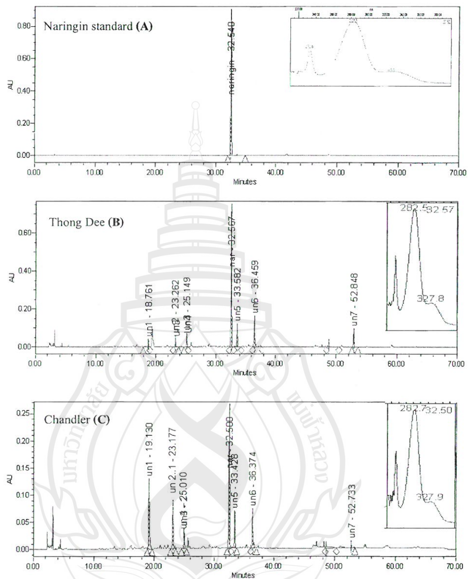
Figure 4.14: HPLC Chromatogram of naringin standard (A), pummelos cvs. “Thong Dee” (B) and “Chandler” (C) at 28 weeks after full bloom
