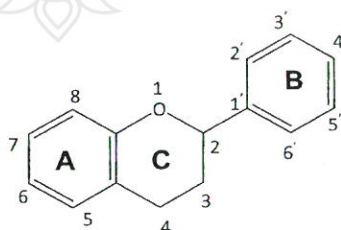
Figure 2.5: The basic structure of flavonoids
