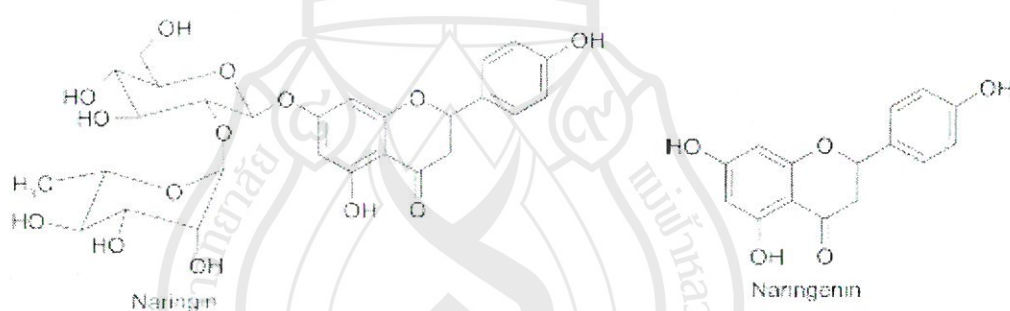
Figure 2.8: The structure of naringin and naringenin.
