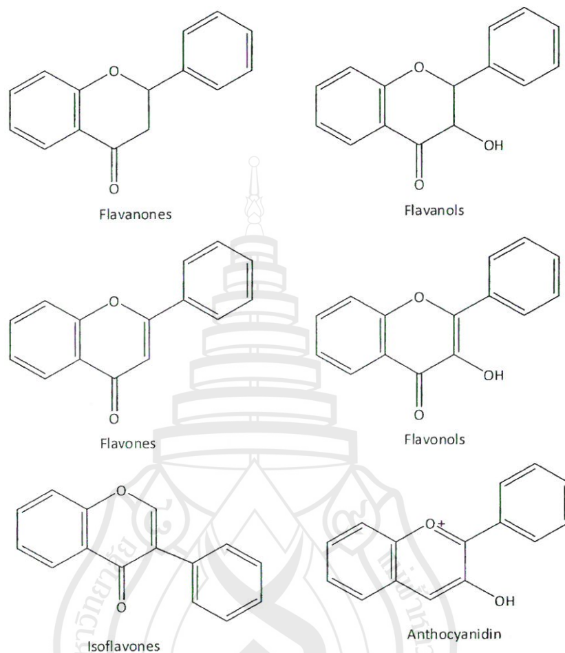
Figure 2.7: The basic structure of flavonoid compounds includes flavanones, flavanols, flavones, isoflavone, and anthocyanidin (Pietta, 2000)
