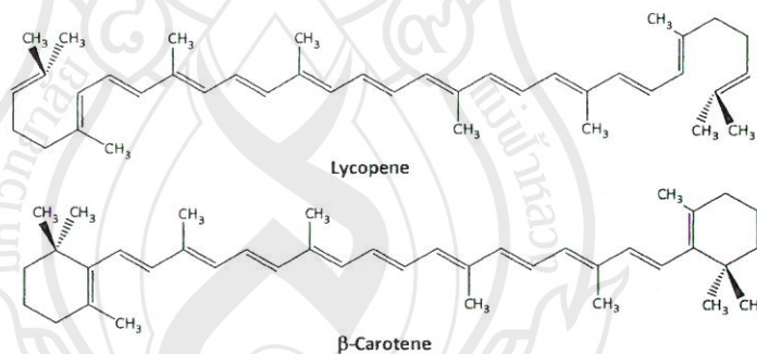
Figure 2.10: The structure of lycopene and \beta -carotene
