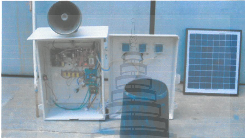
Figure 6 Device model
