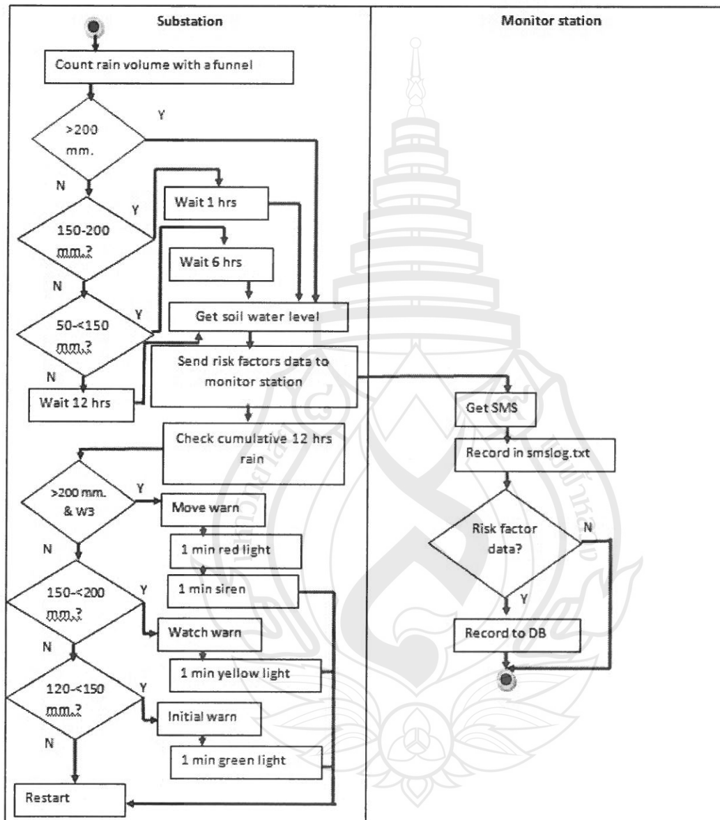
Figure 4 Data transferring function's diagram
