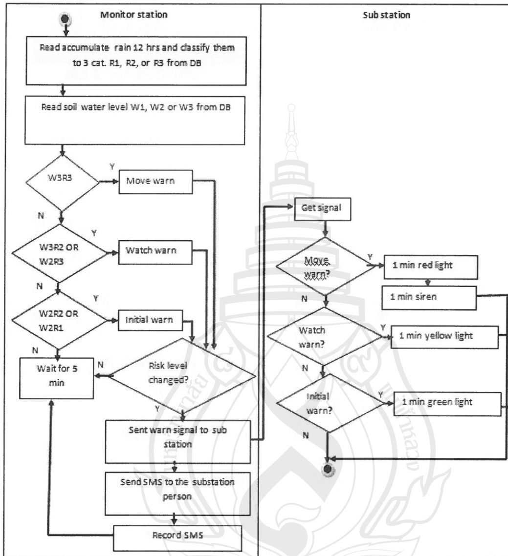
Figure 5 Monitoring and warning system's diagram
